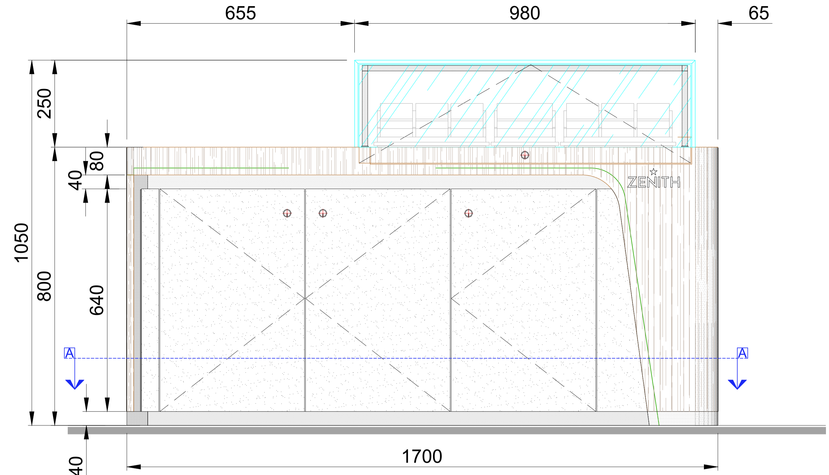
FRONT VIEW COUNTER Pad
