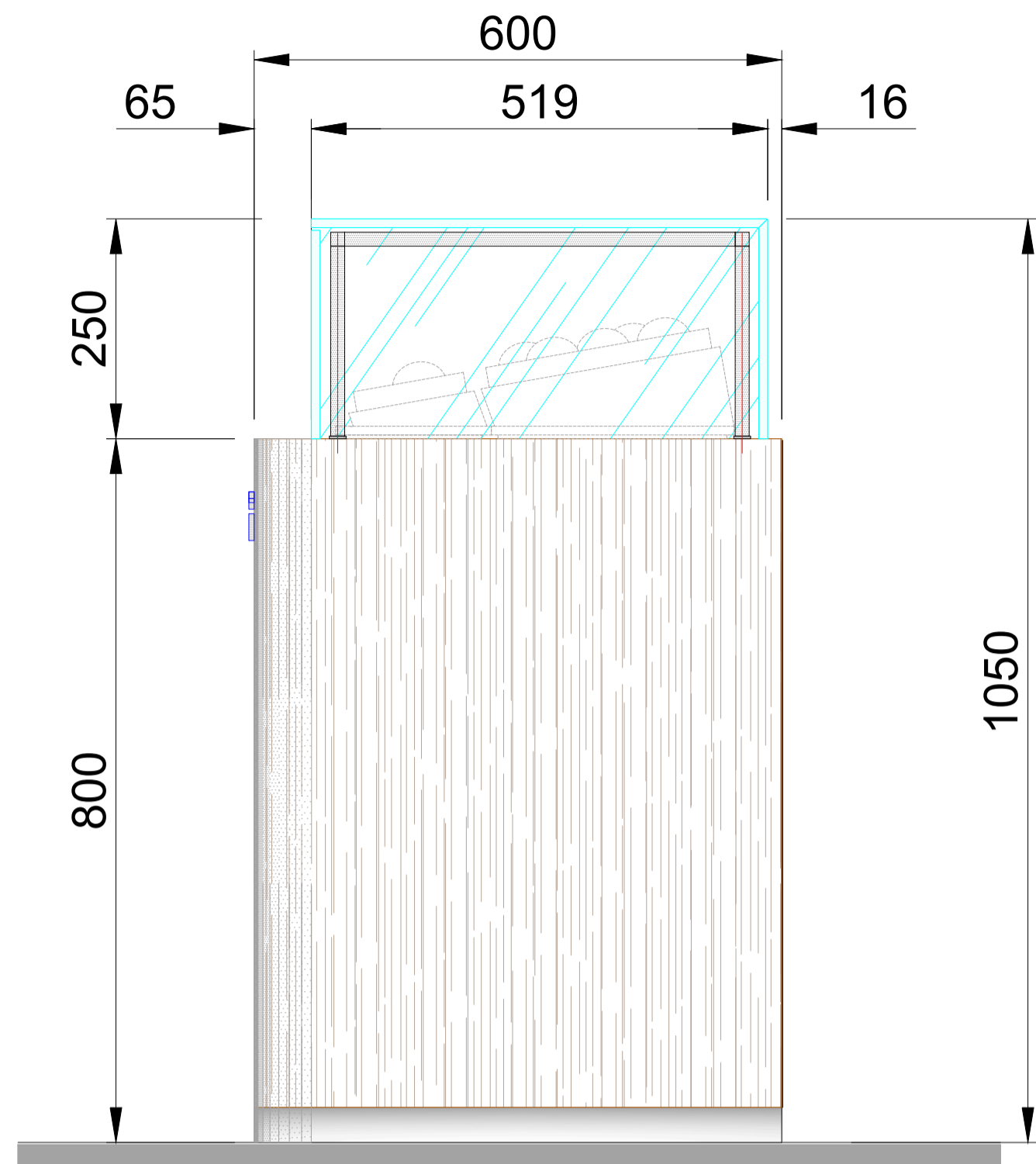
Side VIEW 1 Lateral View - R / COUNTER Pad
