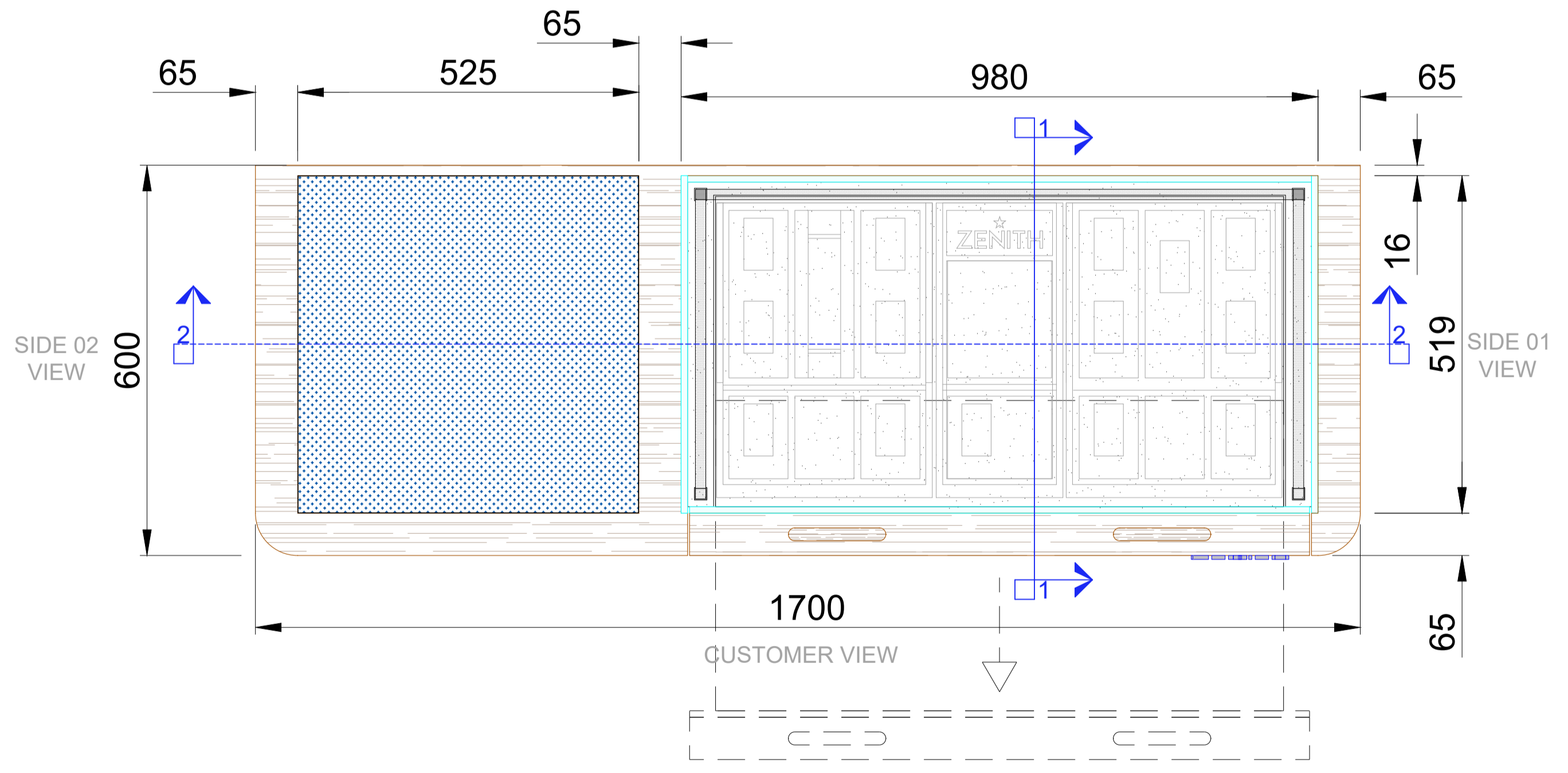
PLAN VIEW COUNTER Pad
