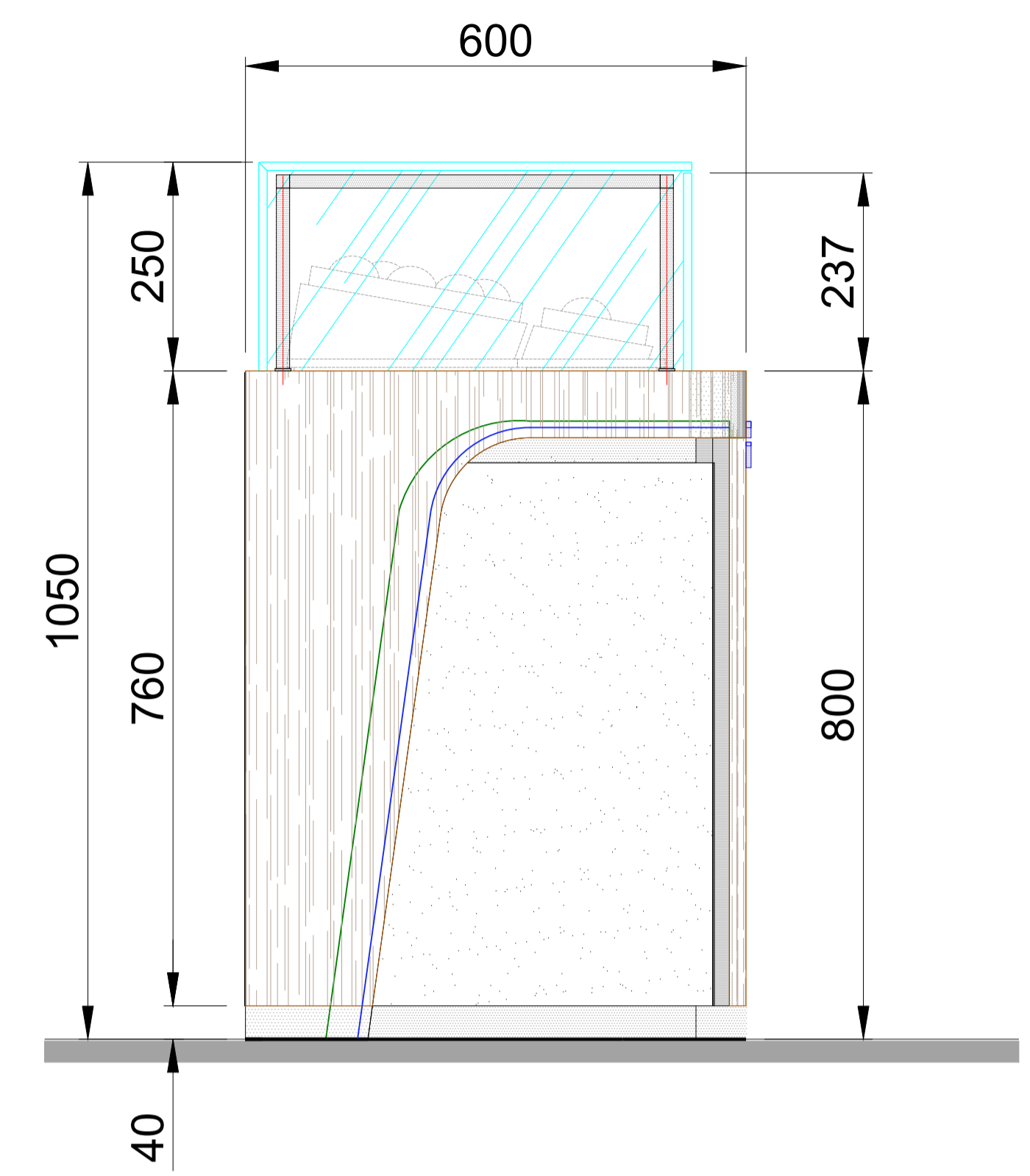
Side VIEW 2 Lateral View - L / COUNTER Pad
